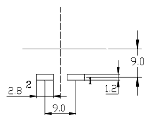
PCB PATTERN
