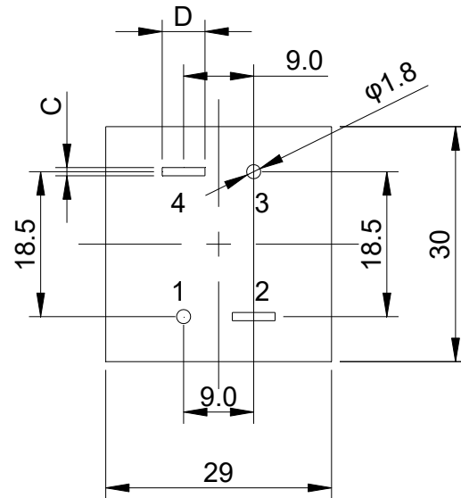
PCB PATTERN
