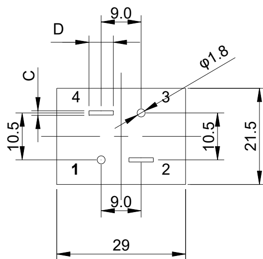
PCB PATTERN
